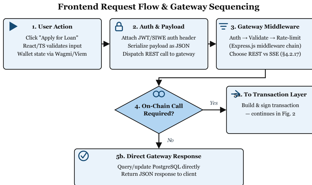
Figure 4.5: Frontend request flow and gateway sequencing.
