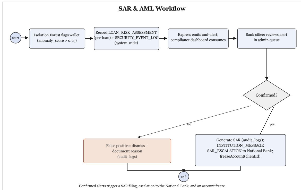
Figure 4.44: SAR and AML workflow.
