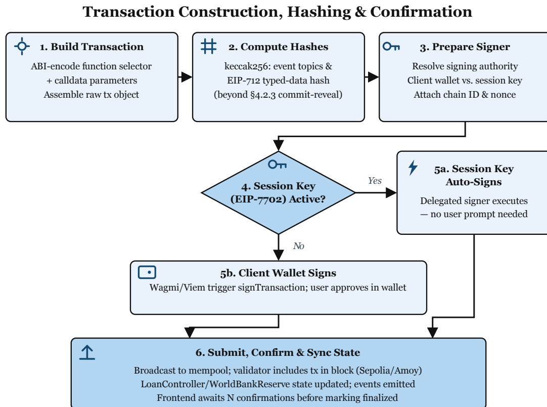
Figure 4.6: Transaction construction, hashing, and confirmation.
